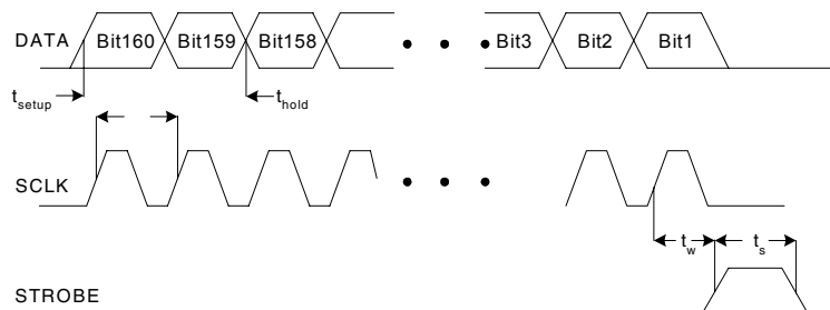
Figure 2. Timing Diagram for Programming the ICS309
