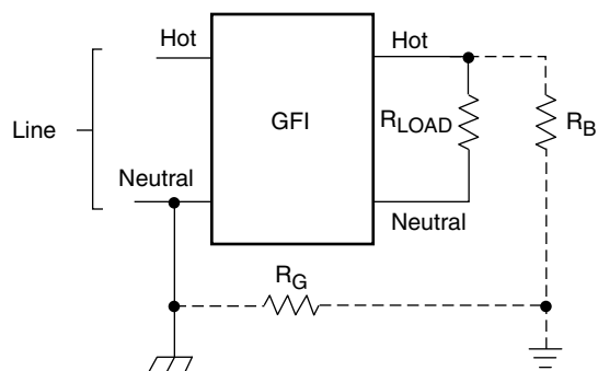
Figure 1. Normal Fault
