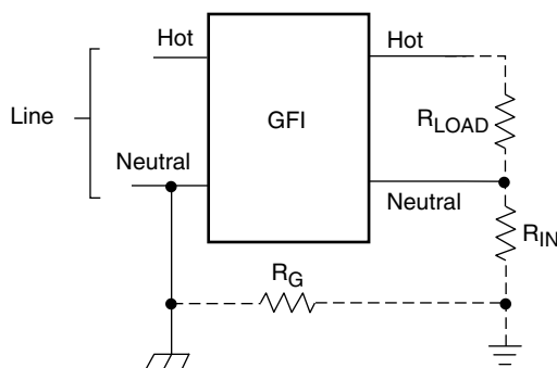
Figure 2. Grounded Neutral Fault
