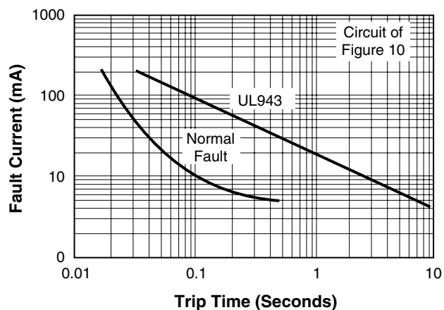
Figure 4. Average Trip Time vs. Fault Current
