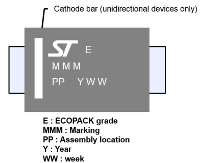
Figure 19. SMA marking
