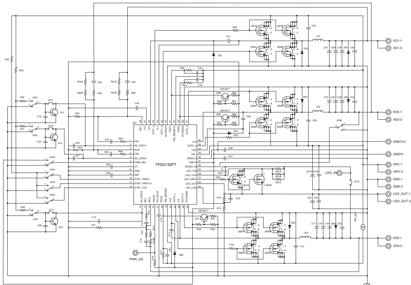
Figure 17. EVM Schematic
