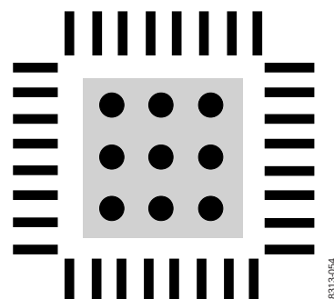
Figure 56. Exposed Pad Layout Example, Top View
