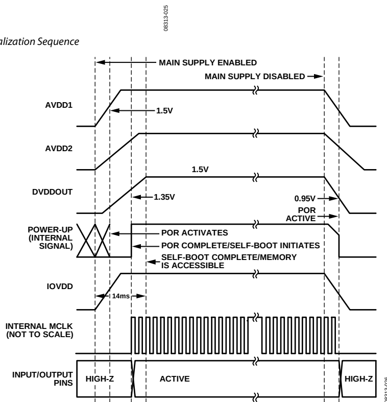
Figure 28. Power-Up and Power-Down Sequence Timing Diagram
