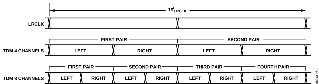
Figure 63. Left First Channel Selection in TDM
