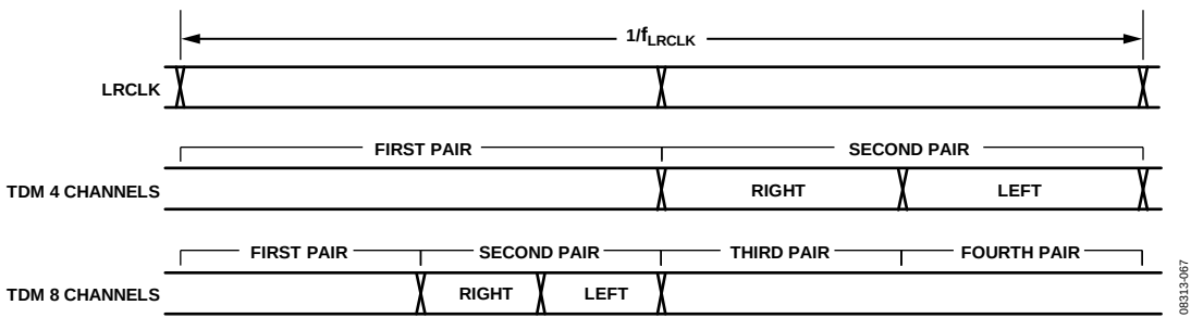
Figure 69. Example of Right Channel First, Second Pair TDM Setting
