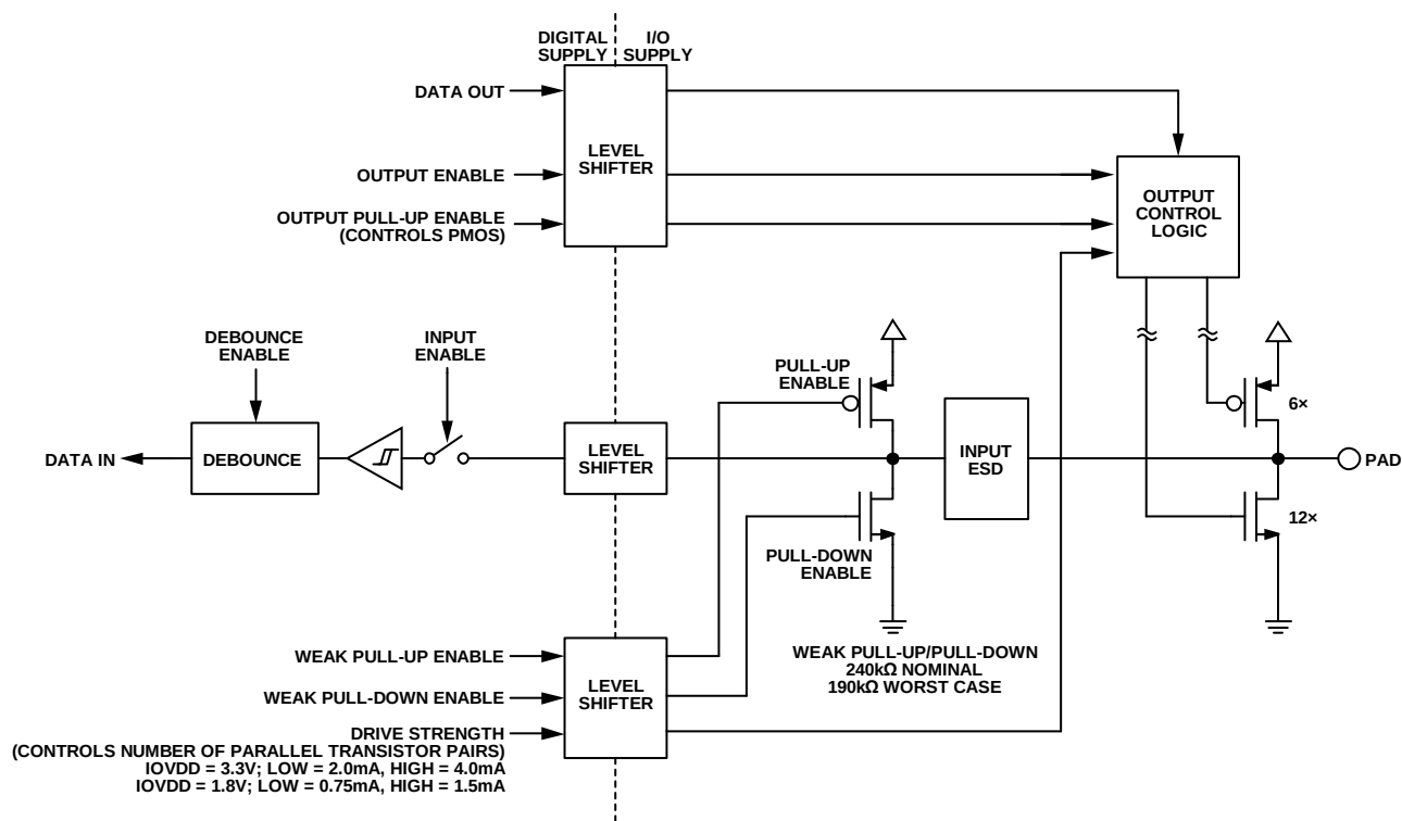
Figure 71. Pad Configuration, Internal Design
