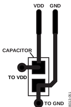
Figure 53. Recommended Power Supply Bypass Capacitor Layout
