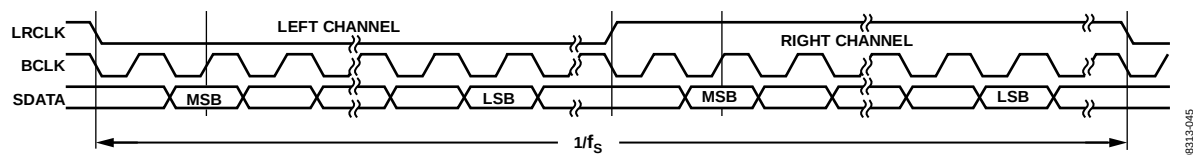
Figure 47. I²S Mode—16 Bits to 24 Bits per Channel
