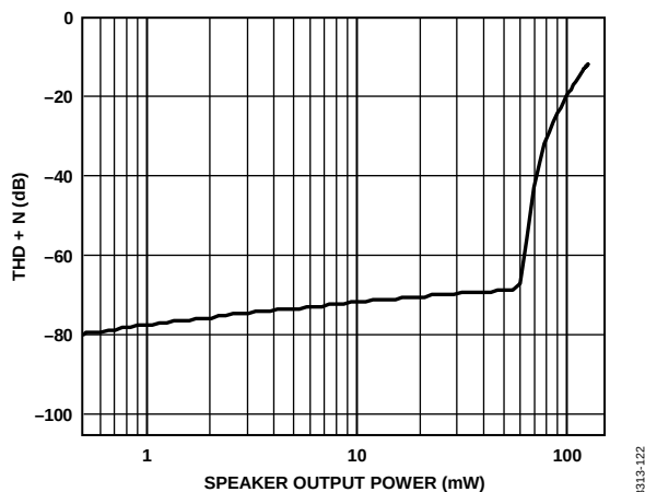
Figure 22. THD + N vs. Speaker Output Power, 8 \Omega Load, 1.8 V Supply
