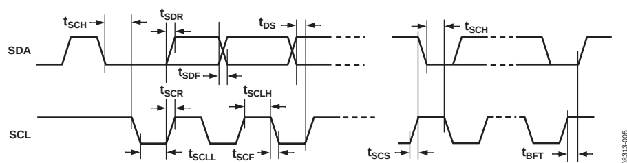
Figure 5. I²C Port Timing
