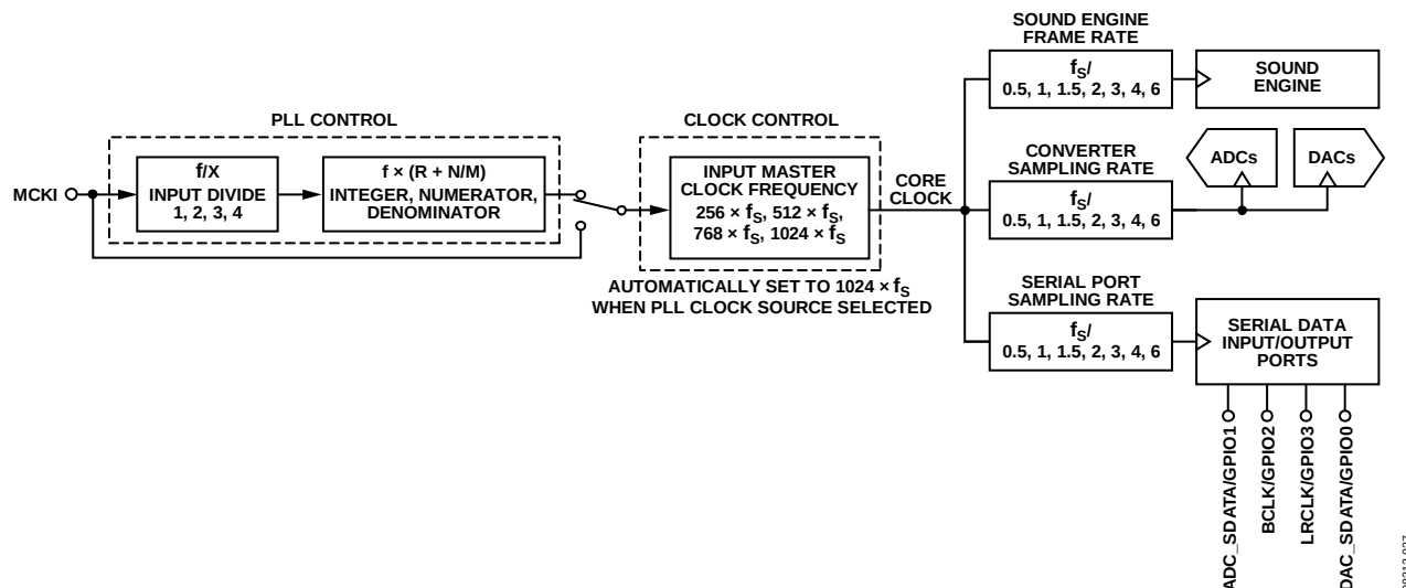
Figure 29. Clock Routing Diagram
