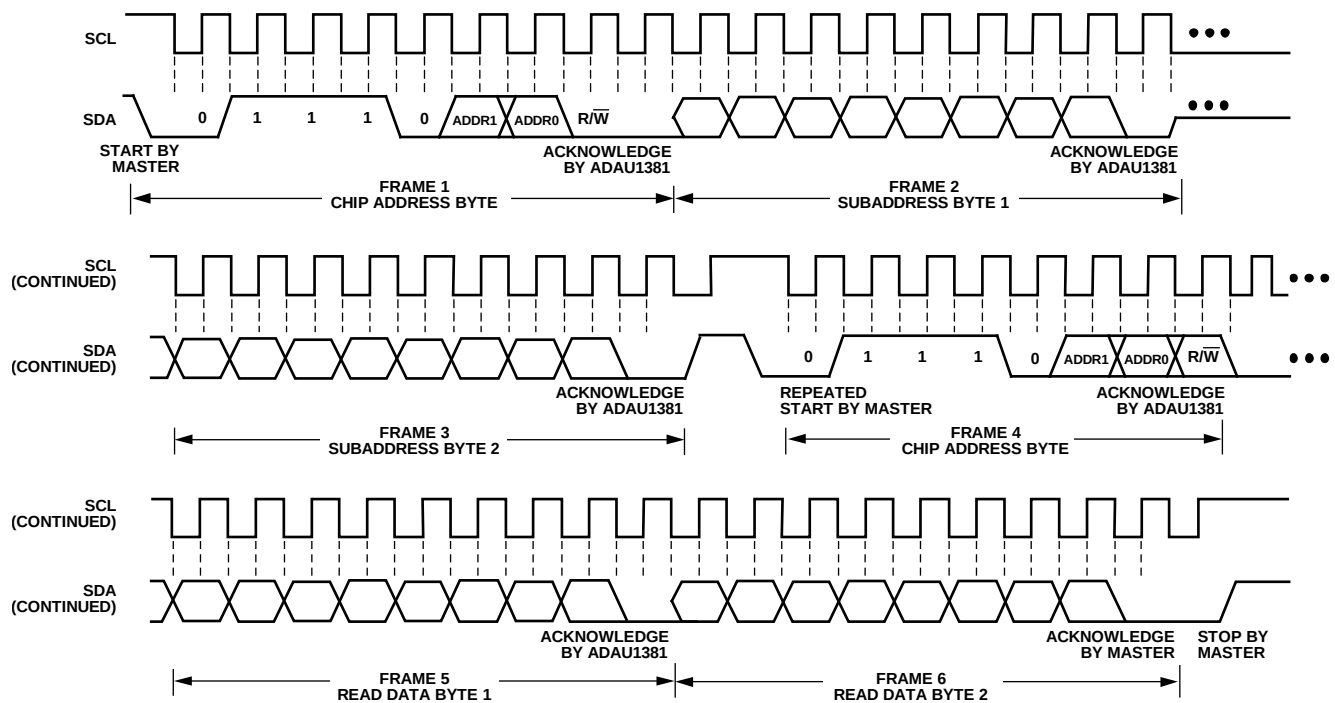
Figure 39. I²C Read from ADAU1381 Clcking
