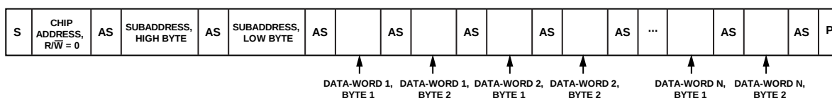
Figure 41. Burst Mode I 2 C Write Sequence
