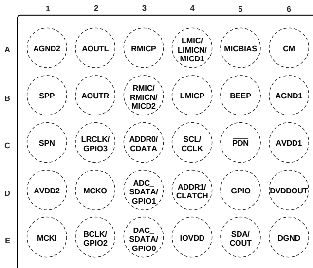
Figure 8. 30-Ball, 6 x 5 WLCSP Pin Configuration (Bottom View)
