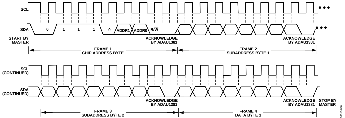
Figure 38. I²C Write to ADAU1381 Clcking
