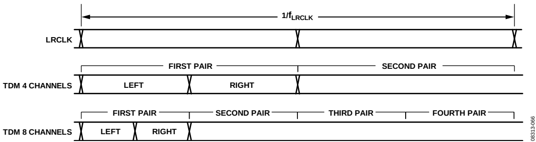
Figure 68. Example of Left Channel First, First Pair TDM Setting
