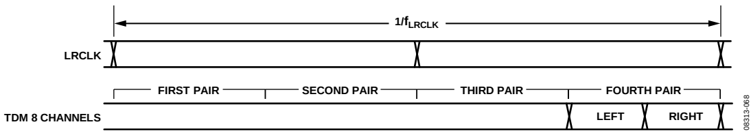
Figure 70. Example of Left Channel First, Fourth Pair TDM Setting
