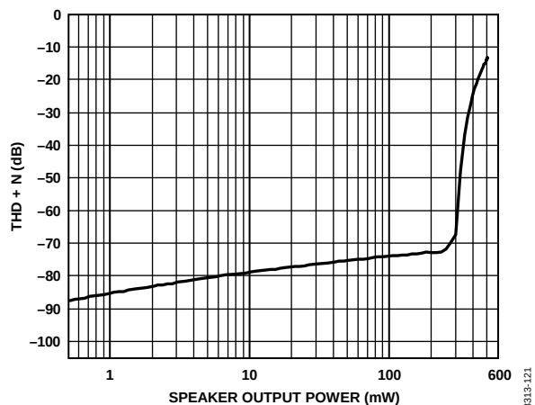
Figure 21. THD + N vs. Speaker Output Power, 8 \Omega Load, 3.3 V Supply
