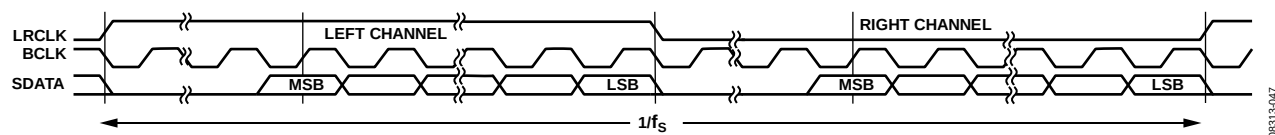
Figure 49. Right-Justified Mode—16 Bits to 24 Bits per Channel
