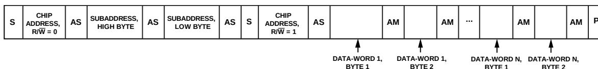
Figure 43. Burst Mode I 2 C Read Sequence
