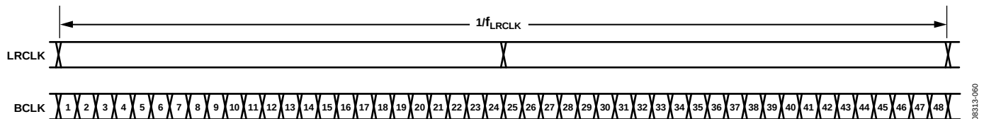
Figure 62. Example: 48 BCLK Cycles per Frame
