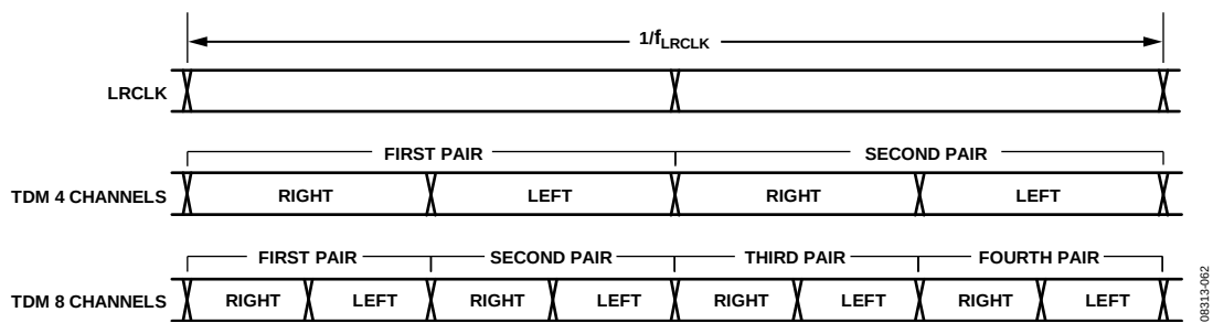
Figure 64. Right First Channel Selection in TDM
