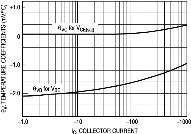
Figure 4. Temperature Coefficients
