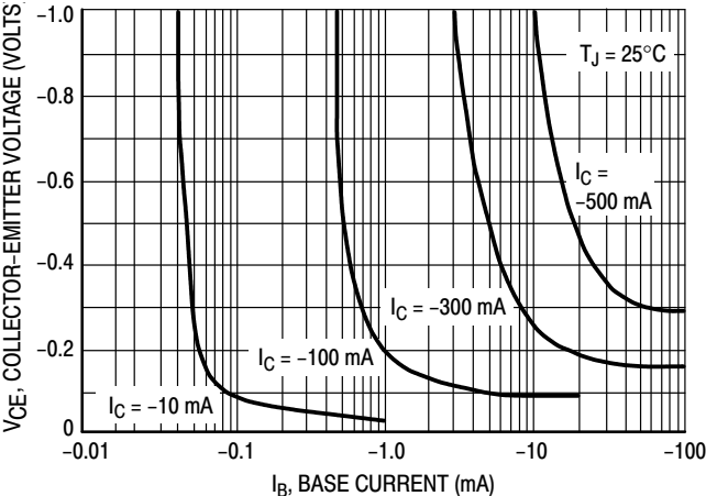
Figure 2. Saturation Region
