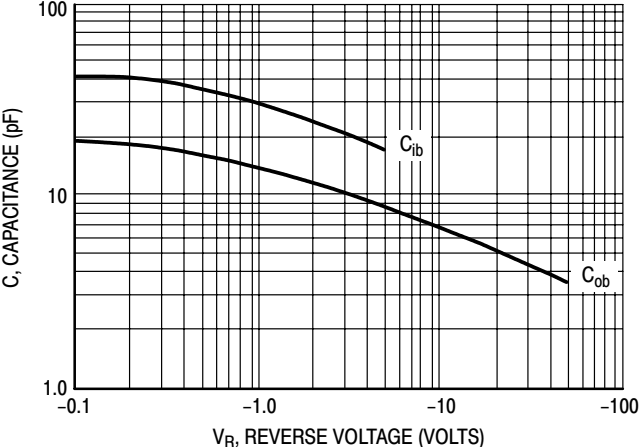
Figure 5. Capacitances
