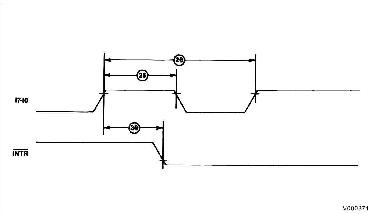
Figure 25 : Interrupt Timing.
