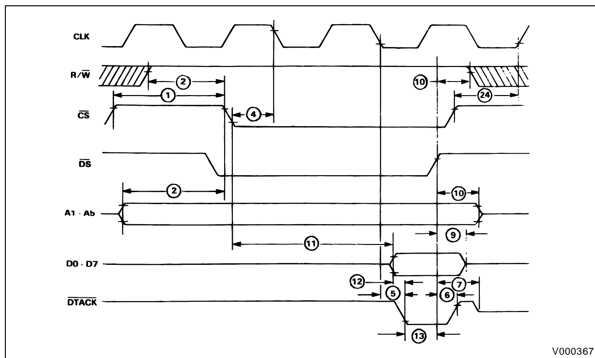
Figure 22 : Write Cycle.
