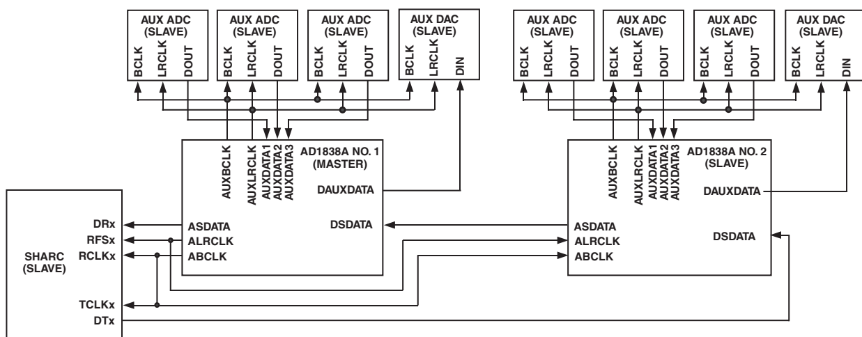
Figure 14. Dual AD1838A Cascade
