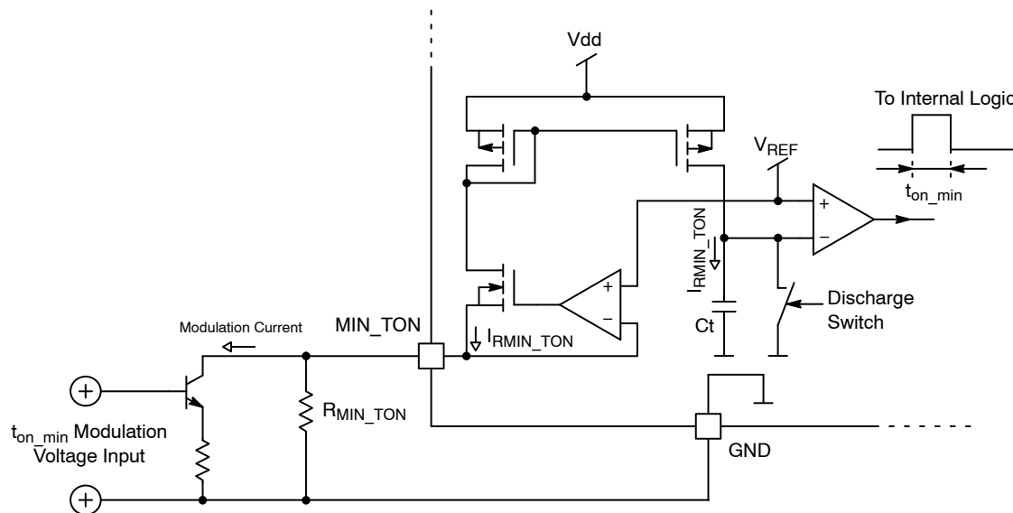
Figure 64. Possible Connection for t_{on\ min} and t_{off\ min} Modulation
