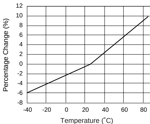
Relative Series Resistance Change vs. Temperature
