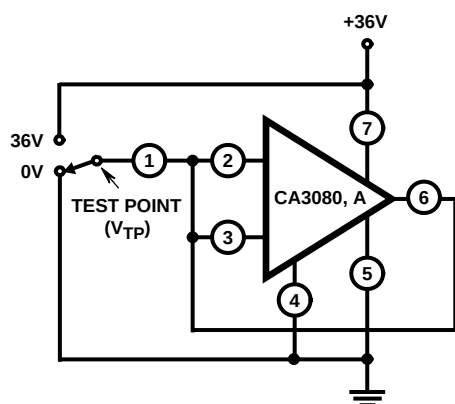
FIGURE 22. LEAKAGE CURRENT TEST CIRCUIT
