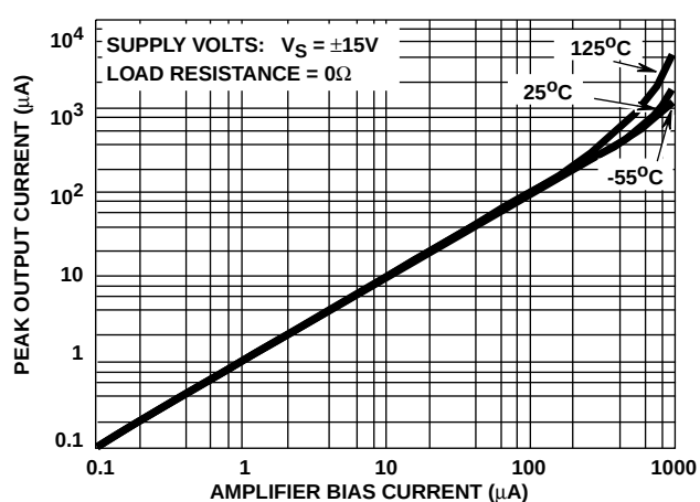
FIGURE 17. PEAK OUTPUT CURRENT vs AMPLIFIER BIAS CURRENT
