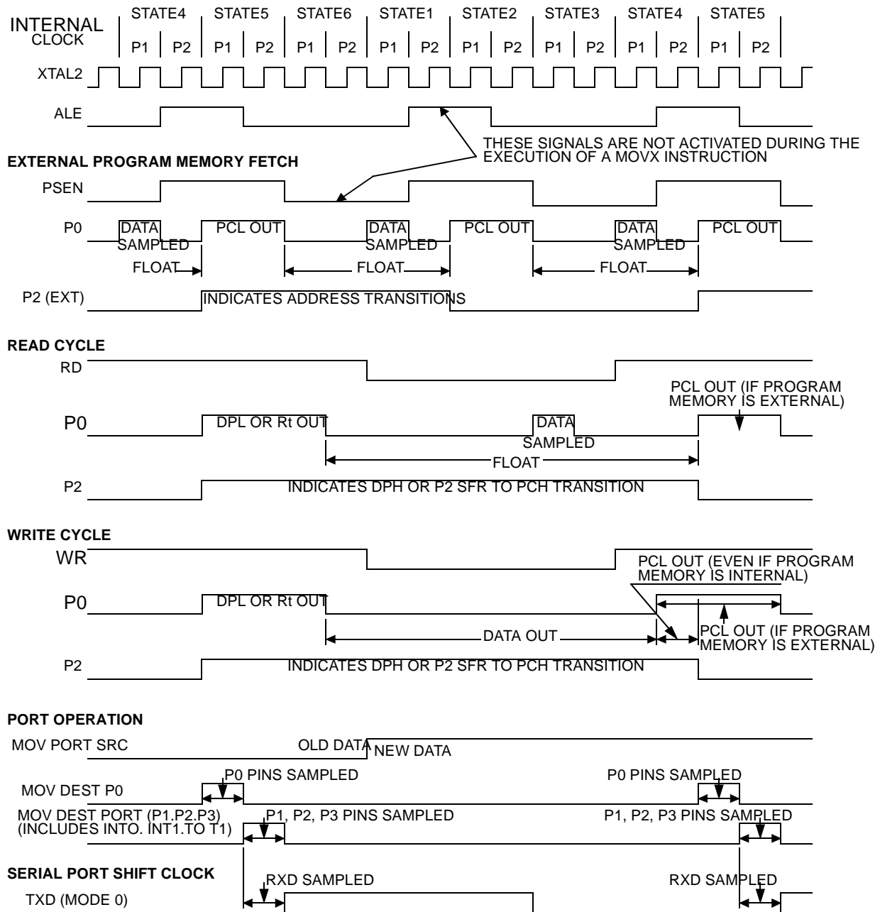
Figure 44. Clock Waveforms
