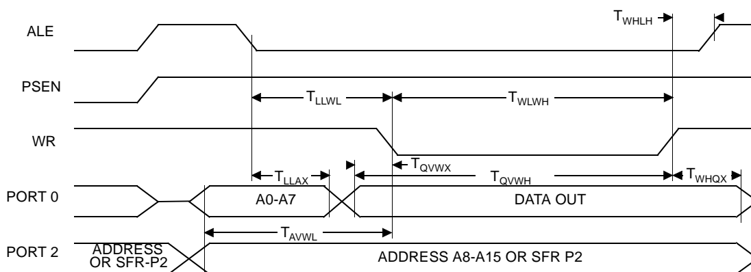
Figure 37. External Data Memory Write Cycle
