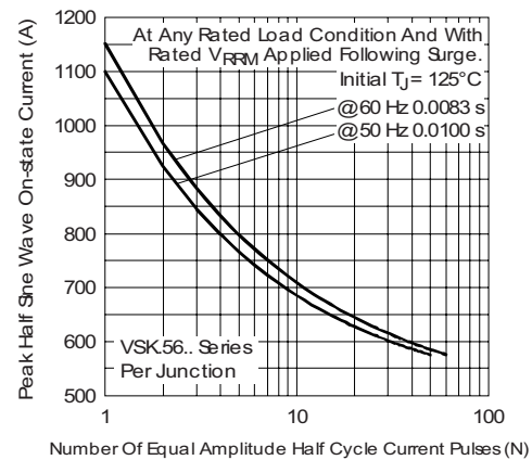
Fig. 14 - Maximum Non-Repetitive Surge Current
