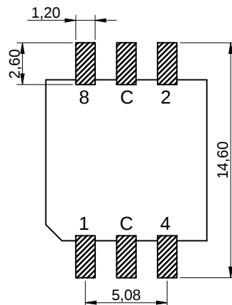
RECOMMENDED LAYOUT
