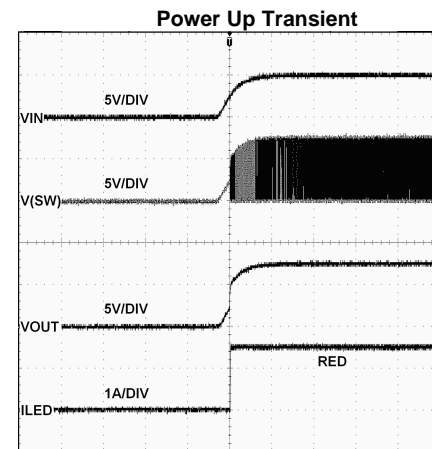
Figure 17. (10ms/DIV)
