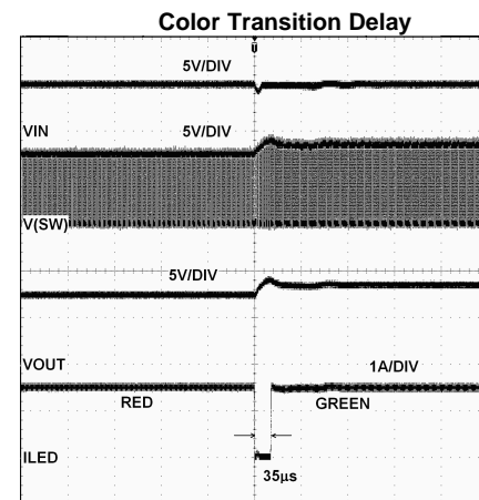
Figure 19. (100µs/DIV)
