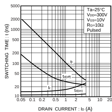
Fig.12 Switching characteristics
