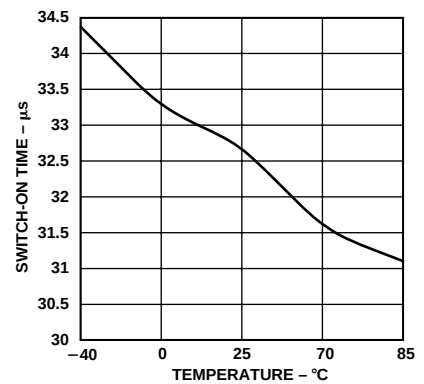
Figure 10. Switch ON Time vs. Temperature
