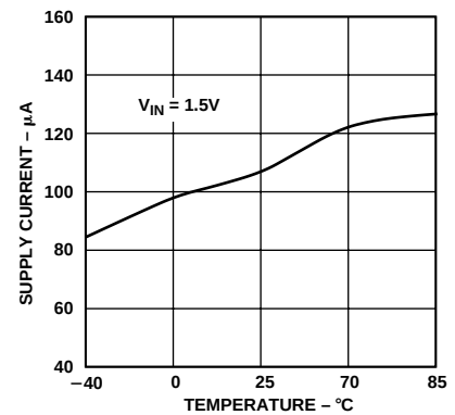
Figure 7. Supply Current vs. Temperature
