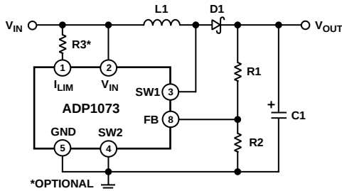
Figure 15. Step-Up Mode Operation
