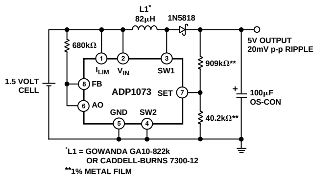
Figure 40. 1.5 V to 5 V Low Noise Step-Up Converter
