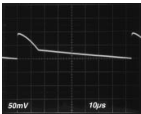
Figure 12. Aluminum Electrolytic
