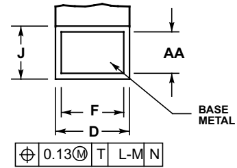
SECTION J1-J1
