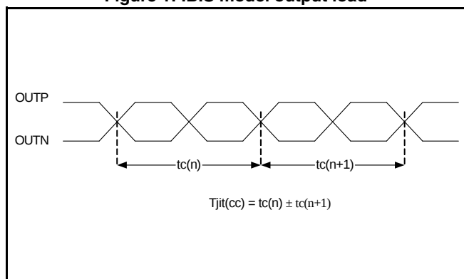
Figure 3: Cycle-cycle jitter
