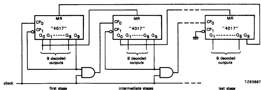
Fig.10 Counter expansion
