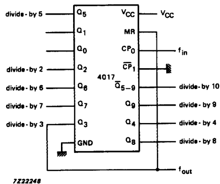
Fig.11 Divide-by 2 through divide-by 10.
