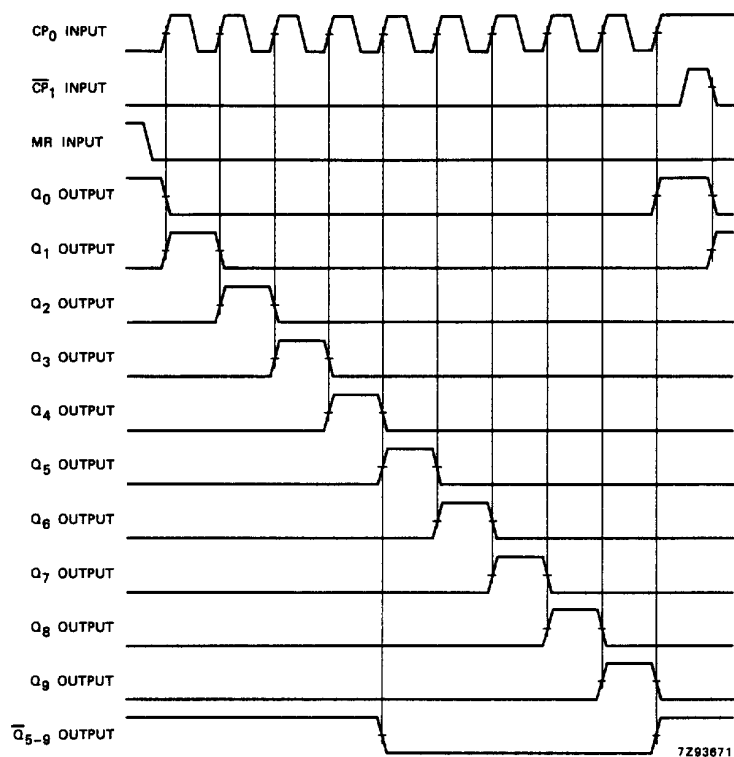
Fig.6 Timing diagram.
