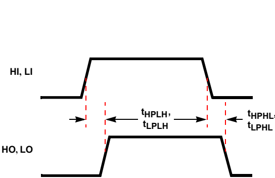
FIGURE 5. PROPAGATION DELAYS
