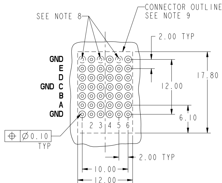
RECOMMENDED PCB HOLE PATTERN (COMPONENT SIDE)
