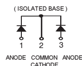
Case Outline and Dimensions - TO-254AA
