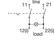
2-pole, unprotected
