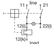
2-pole, unprotected
