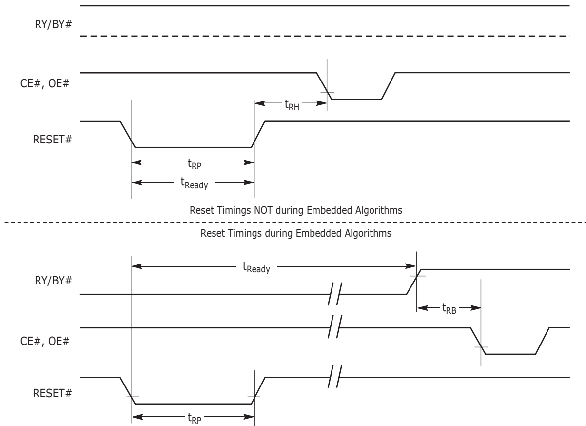
Figure I4. RESET# Timings
