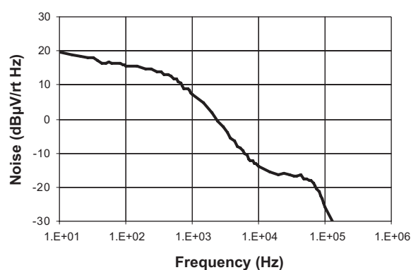
AAT3200 Noise Spectrum
