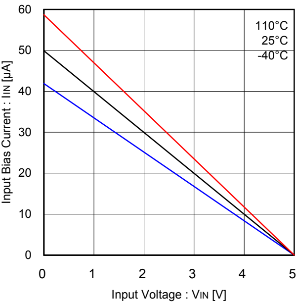
Figure 39. Input Bias Current (CCW, FGS)
