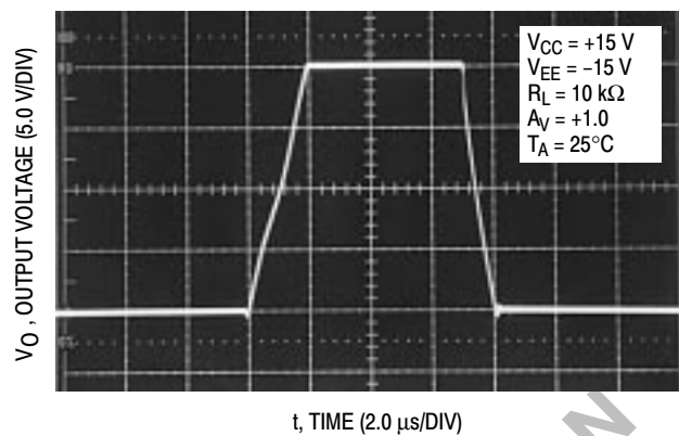
Figure 28. Transient Response
