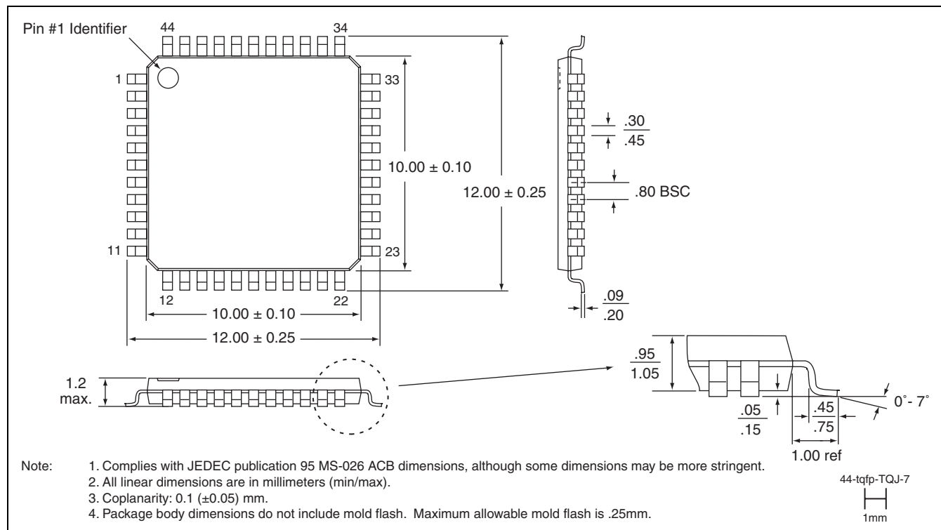
44-LEAD THIN QUAD FLAT PACK (TQFP) SST PACKAGE CODE: TQJ
