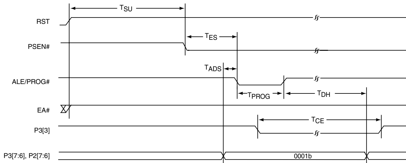
FIGURE 13-16: CHIP-ERASE
