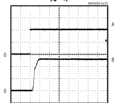
MAX5035DUSA STARTUP WAVEFORM ( I_O = 0 )
