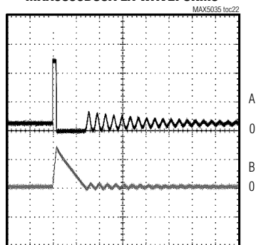
MAX5035DUSA LX WAVEFORMS
