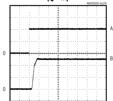
MAX5035DUSA STARTUP WAVEFORM ( I_O = 1A )
