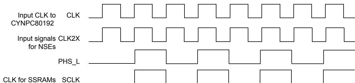
Figure 5-1. NDC Clocks
