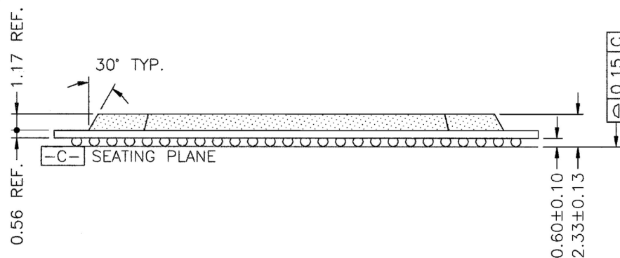
Figure 20-2. Package Side View
