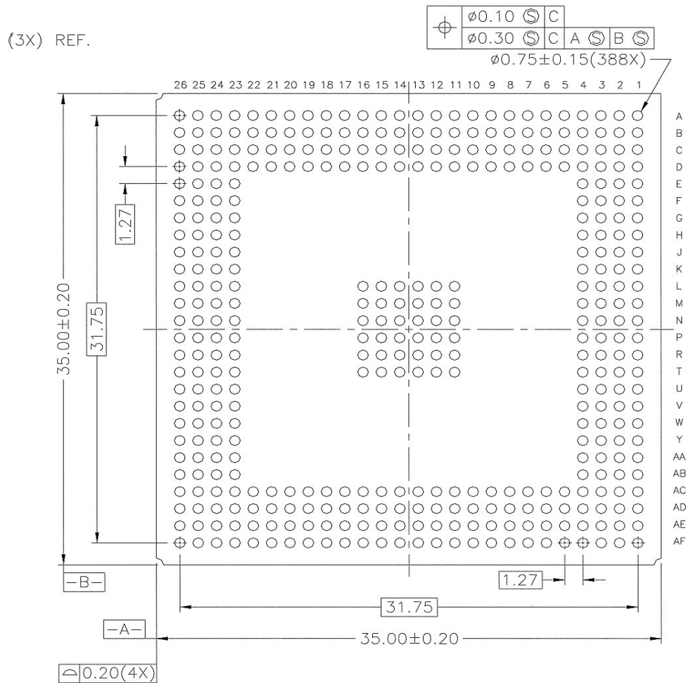
Figure 20-1. Package Bottom View
