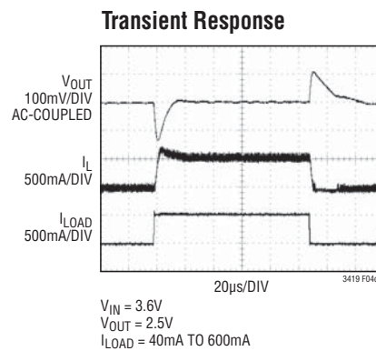
Figure 4c. Transient Response
