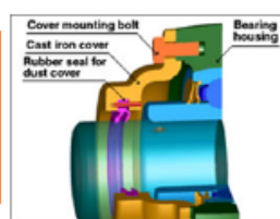
Fig.B Cast iron covered bearing unit Cast iron covered bearing unit
