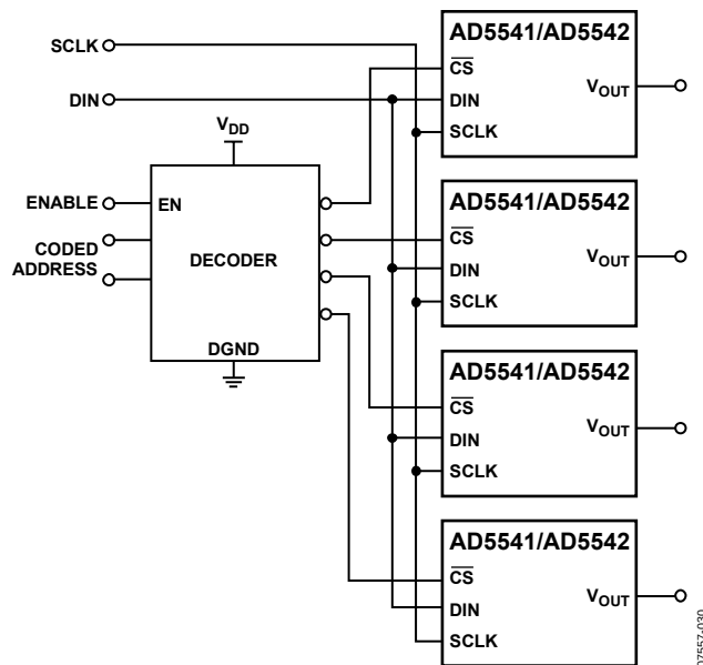
Figure 36. Addressing Multiple AD5541/AD5542s
