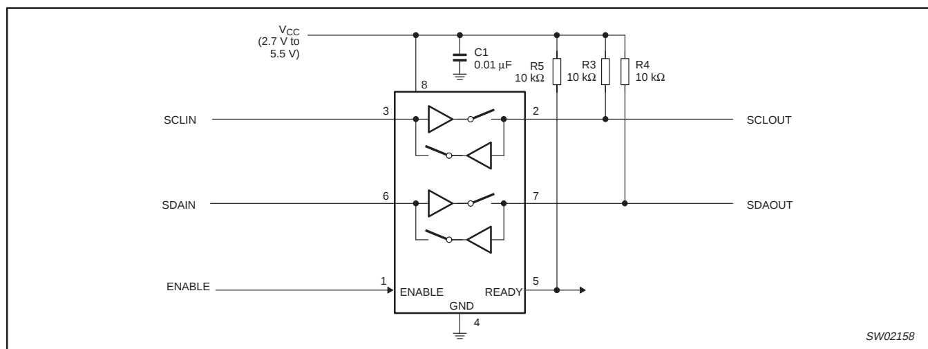
Figure 2. Typical application — PCA9513
