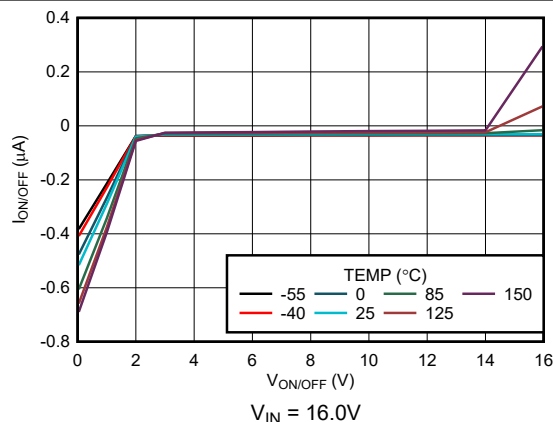
Figure 5-28. ON/OFF Pin Current vs V_{ON/OFF} (New Chip)
