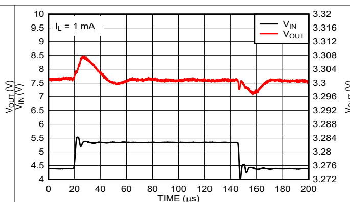
Figure 7-8. Line Transient Response (New Chip)
