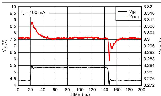
Figure 7-7. Line Transient Response (New Chip)
