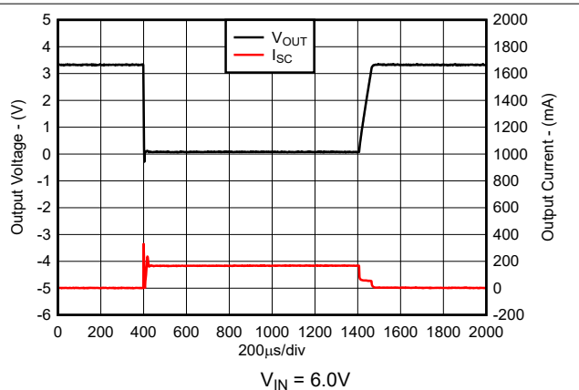
Figure 5-16. Short-Circuit Current vs Time (New Chip)
