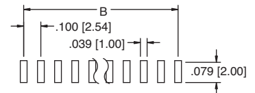
PH1RB-10-UA-SMT
