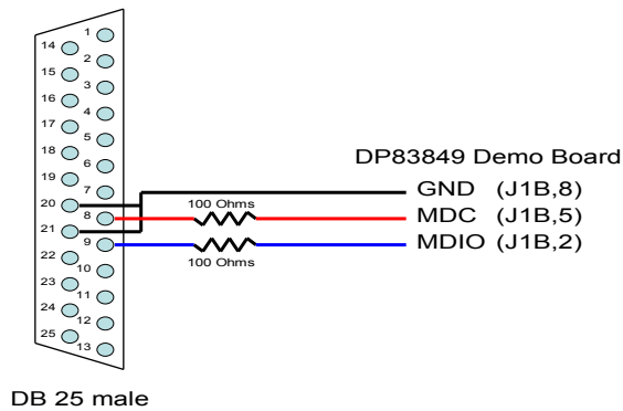
Figure 1. Direct Connect Cable with In Line Resistors
