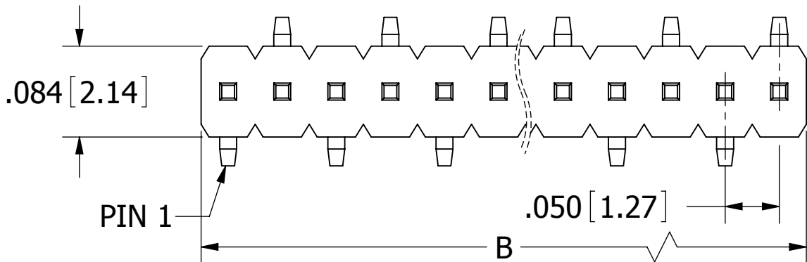
GRP B _ 1 VWTD-RC (OPPOSITE BEND, ONLY APPLICABLE ON EVEN PIN COUNTS)
