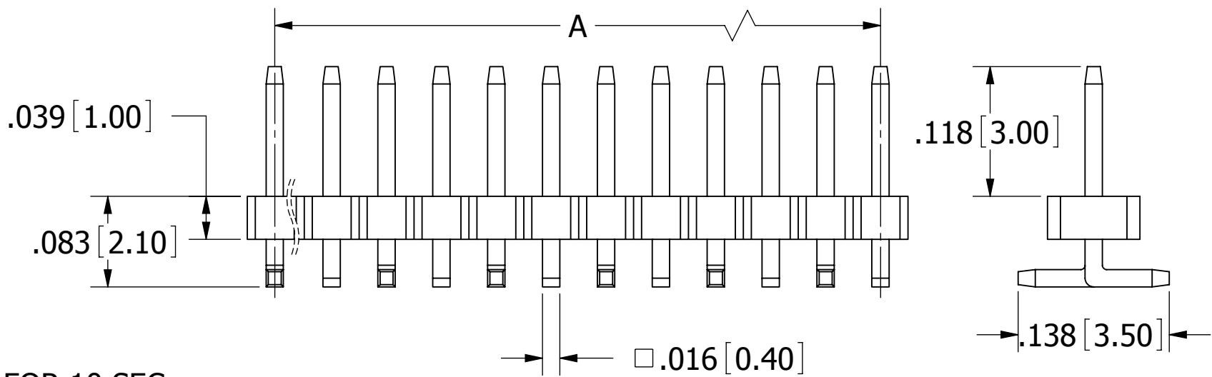
GRP B _ 1 VWTD-RC (OPPOSITE BEND, ONLY APPLICABLE ON EVEN PIN COUNTS)
