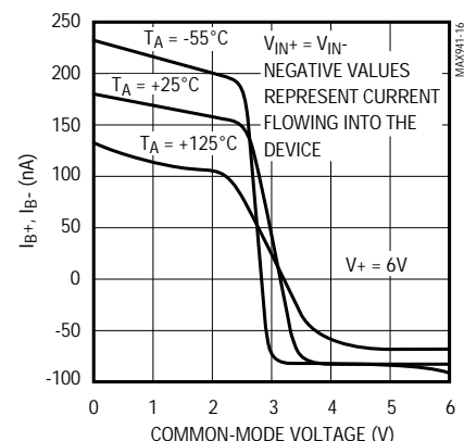
INPUT BIAS CURRENT (IB+, IB-) vs. VCM
