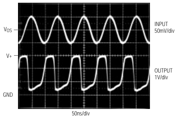
10MHz RESPONSE
