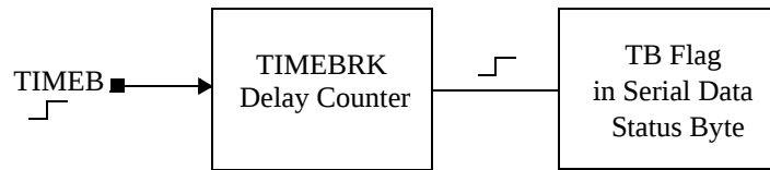
Figure 37. Time Break Block Diagram
