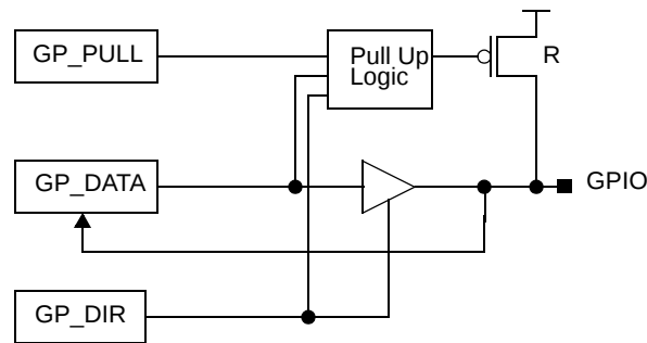
Figure 38. GPIO Block Diagram
