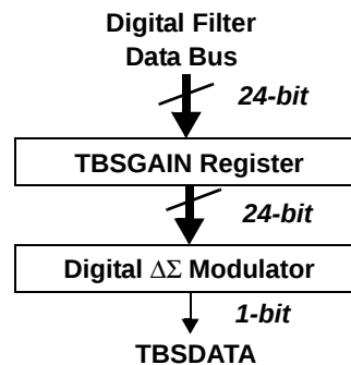
Figure 36. Test Bit Stream Generator Block Diagram
