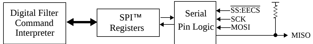
Figure 17. Serial Interface Block Diagram
