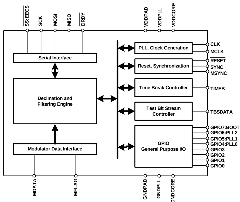
Figure 1. CS5378 Block Diagram
