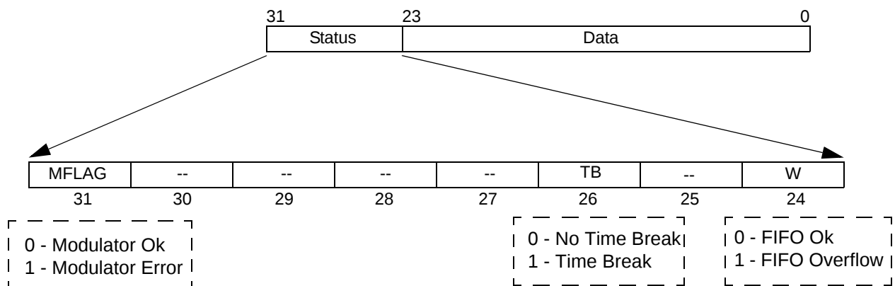
Figure 34. 32-bit Serial Data Format
