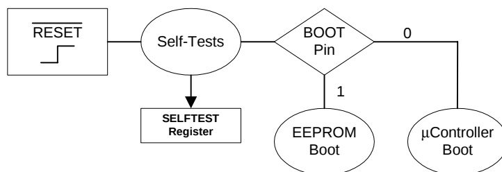
Figure 11. Reset Control Block Diagram
