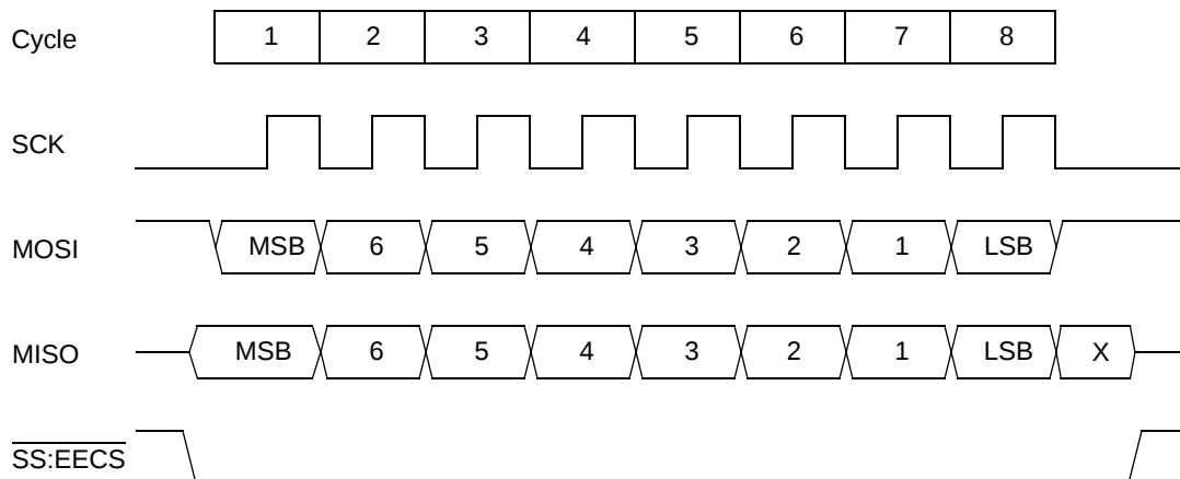
Figure 15. EEPROM Serial Read Transactions
