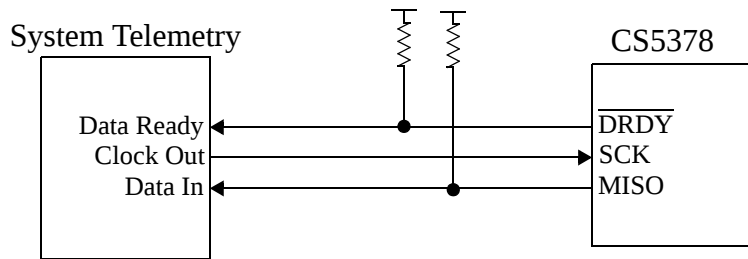
Figure 33. Serial Data Interface Block Diagram
