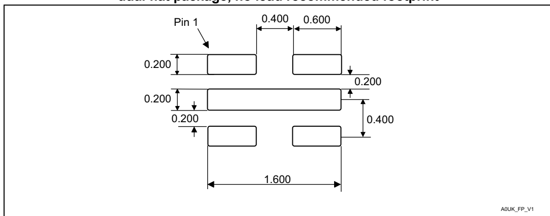
Figure 17. UDFPN5 - 5-lead, 1.7 × 1.4 mm, 0.55 mm thickness, ultra thin fine pitch dual flat package, no lead recommended footprint
