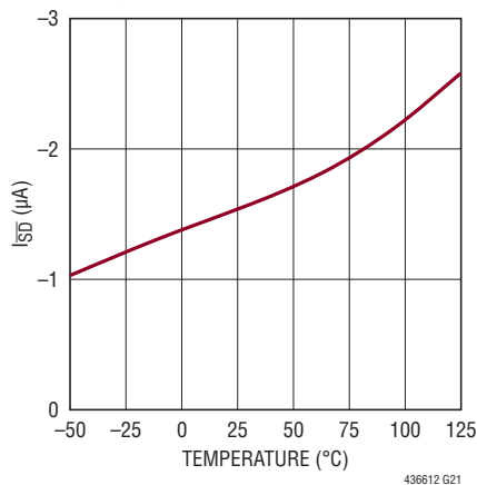
\overline{SD} Pull-Up Current vs Temperature
