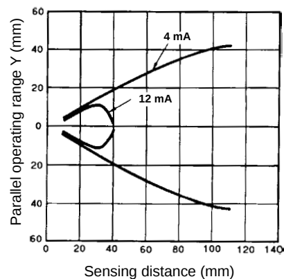
E32-T16 with E3XA-CC4A amplifier and 0.5 mm slit
