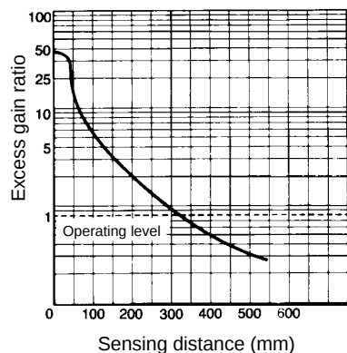
E32-TC50/TC200/TC500/TC1000 with E3X-A11 amplifier
