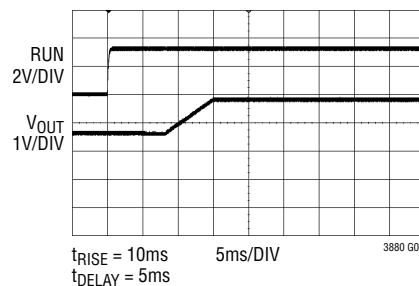
Start-Up into a Pre-Biased Load
