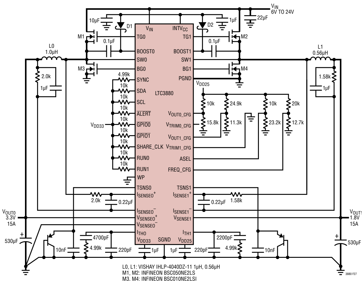
Figure 27. High Efficiency Dual 500kHz 3.3V/1.8V Step-Down Converter
