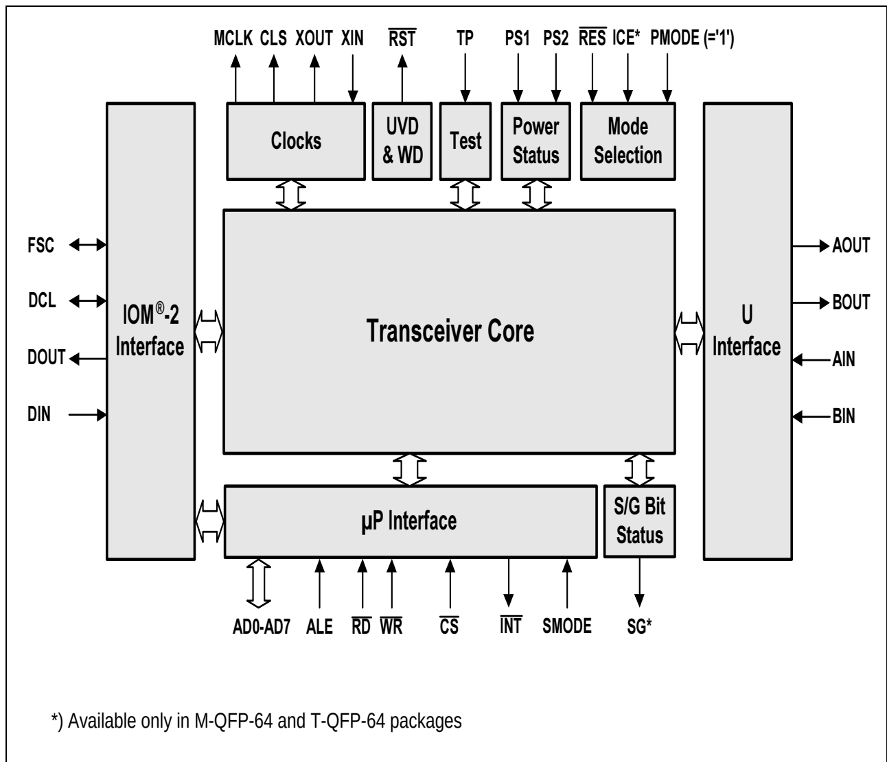
Figure 16 Device Architecture in \mu P Mode
