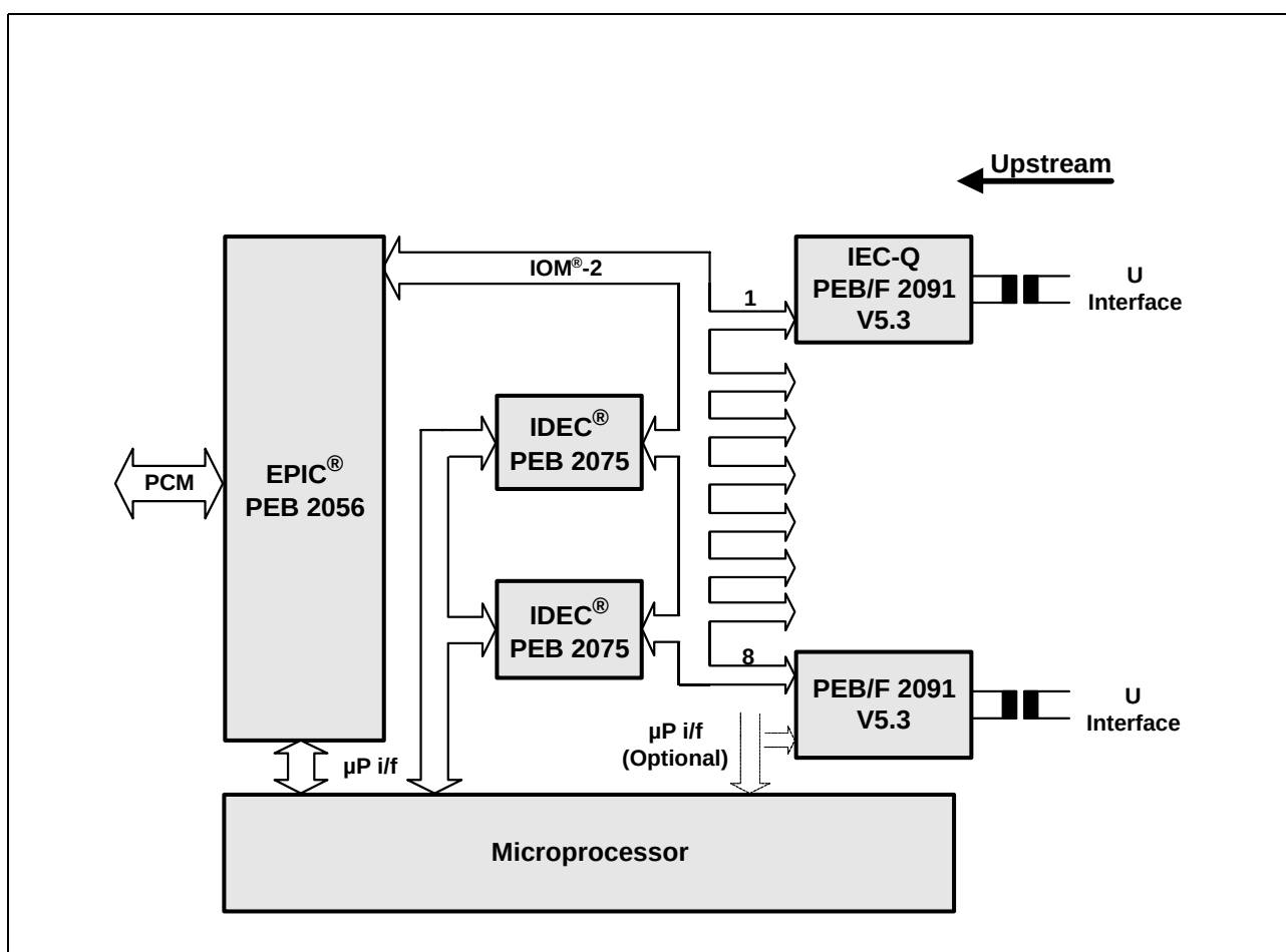
Figure 11 LT and Access Network Applications
