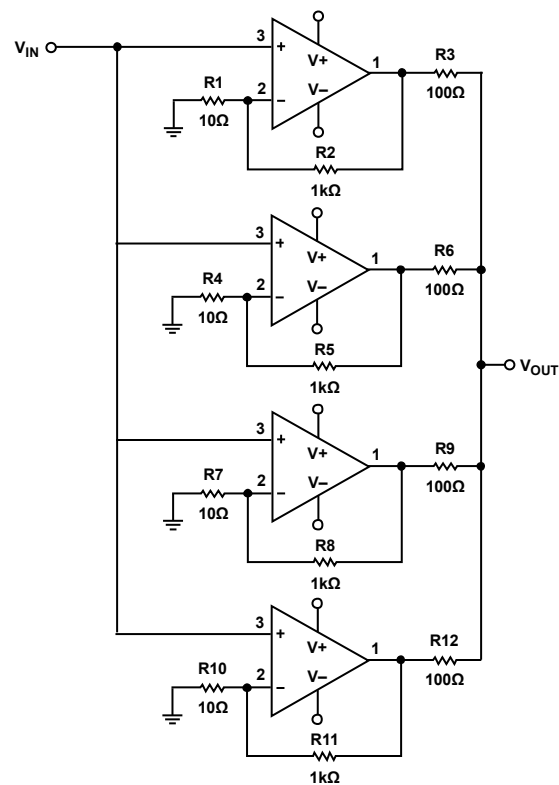
Figure 43. Noise Reduction
