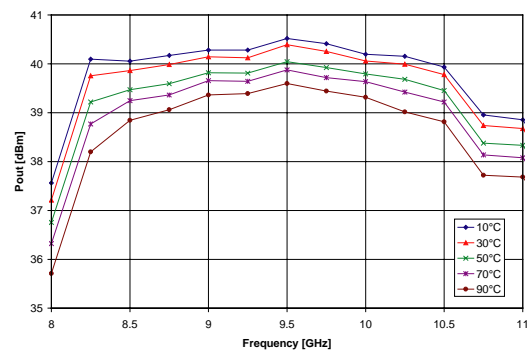
Output power
