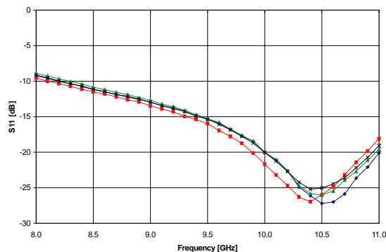
Input return loss (V d =8V, V gg =-5V)
