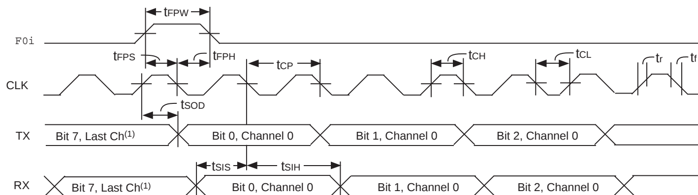
Figure 8. GCI Timing
