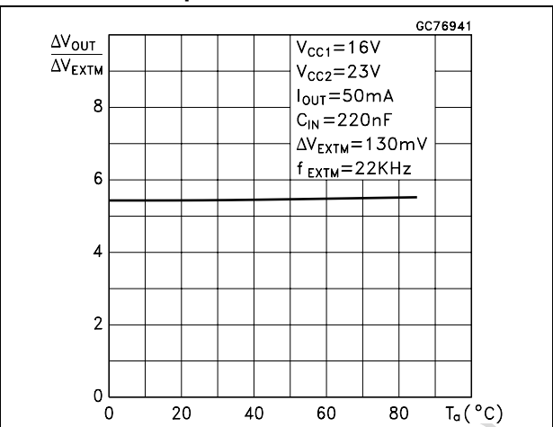
Figure 10. External modulation vs temperature
